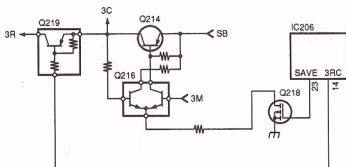
Fig. 13 Battery save circuit
