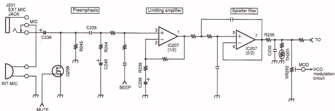
Fig. 5 Microphone amplifier
